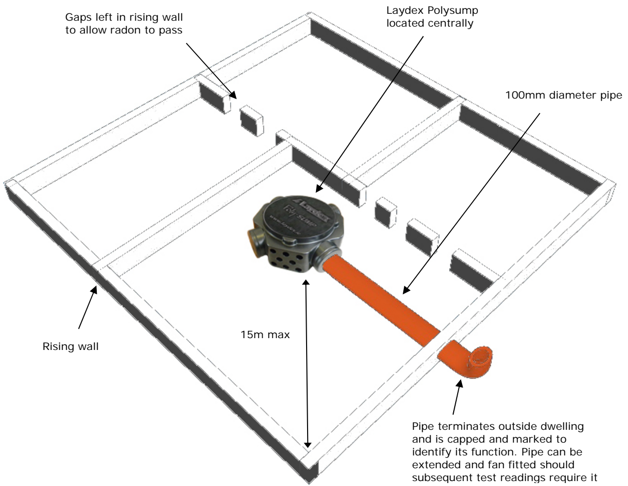
Figure 1: Sump layout
